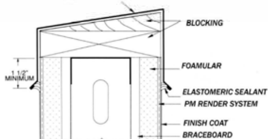
R1.01 PARAPET FLASHED PRIOR TO COATING
